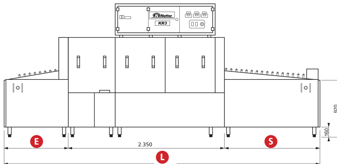
VISTA FRONTAL
